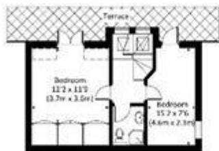
FOURTH FLOOR
